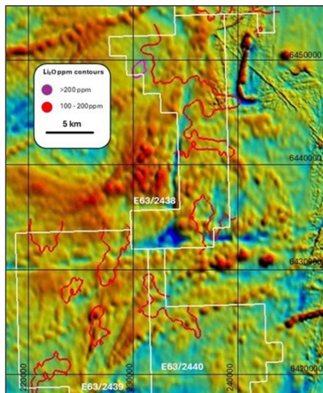
Figure 12: Soil sampling on southern project area showing Li 2 O contours (overlying total magnetic intensity GSWA 1:250,000)
