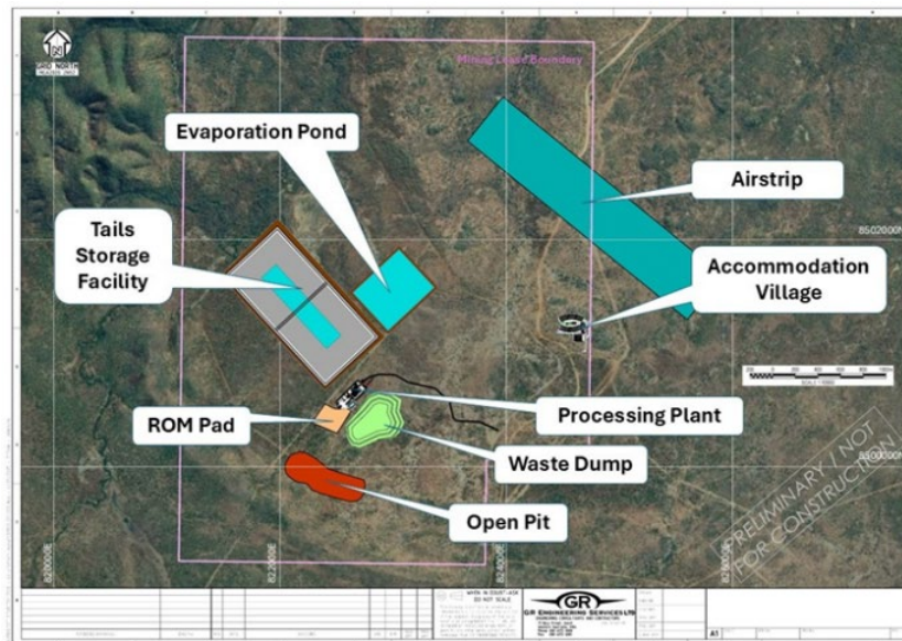
Figure 2 – Overall Leliyn project plan including key infrastructure
